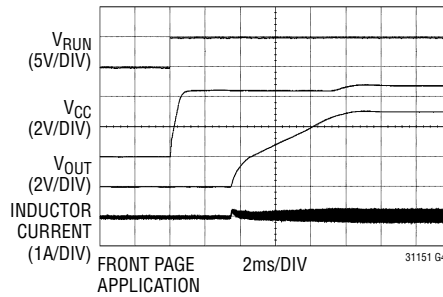
Soft-Start Waveforms
