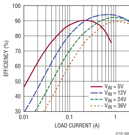
PWM Mode Efficiency, V_{OUT} = 12\text{V} , f_{SW} = 1\text{MHz}
