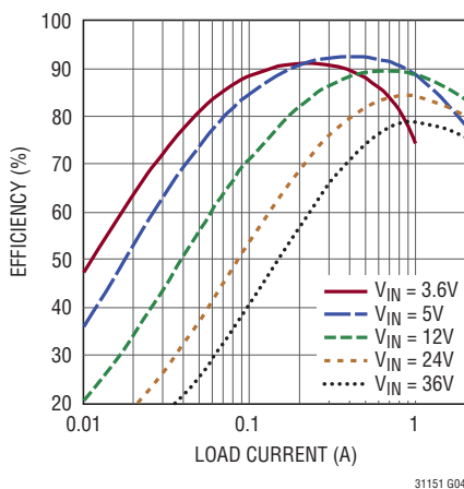
PWM Mode Efficiency, V_{OUT} = 5\text{V} , f_{SW} = 1\text{MHz} , Non-Bootstrapped
