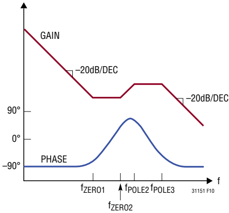
Figure 10. Type III Compensation Bode Plot
