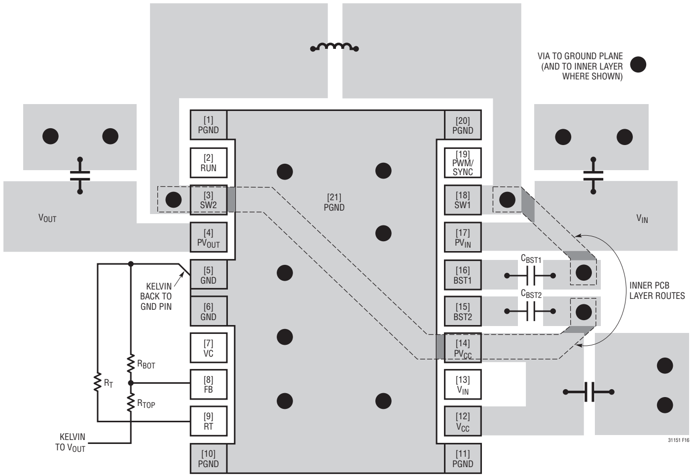
Figure 16. PCB Layout Recommended for the FE Package
